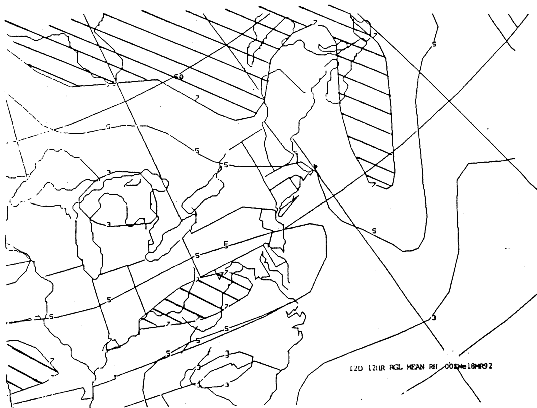
Figure 7. 0000 UTC, March 18, 1992. NGM 1000-500 mb mean relative humidity. Hatched area denotes RH > 70%.
