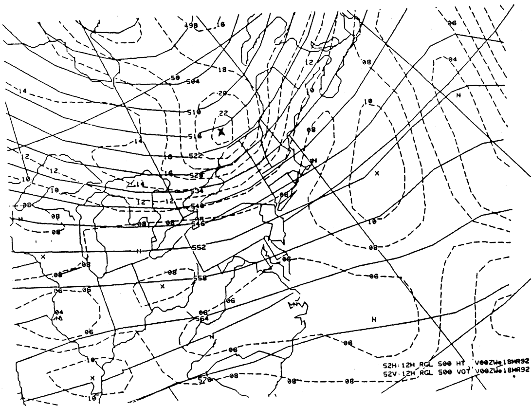
Figure 5. 0000 UTC, March 18, 1992. NGM 500 mb height analysis and vorticity.
