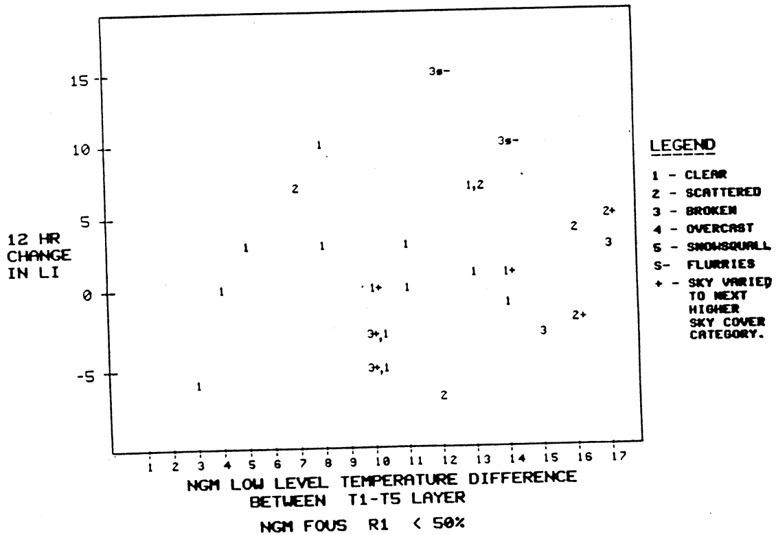
Figure 2. November 1989 through March 1992, WSO Concord, 12-hr change in LI vs. the NGM T1-T5 temperature difference. Boundary layer RH (R1) < 50%.
